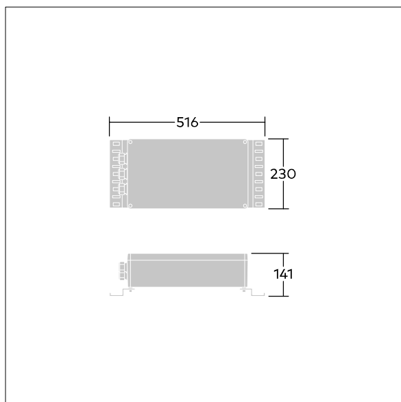
TLG_GTPR_M_GEARBOX_AL.wmf
