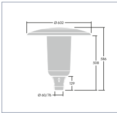
VERSION FINE Ø 60 & Ø 76
